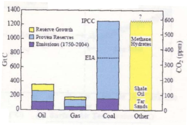
Figure 1. Fossil Fuel Reservoirs, from Figure 6(b) of James Hansen et al., Climate Change and Trace Gases . On the web at: http://www.giss.nasa.gov/~jhansen/docs/RoyalSoc.070218.pdf Note that the scale of CO 2 concentrations on the right side of Figure 1 refers to the change in atmospheric concentration if all of the CO 2 emissions from burning the fossil fuel indicated were to remain in the atmosphere. 11
